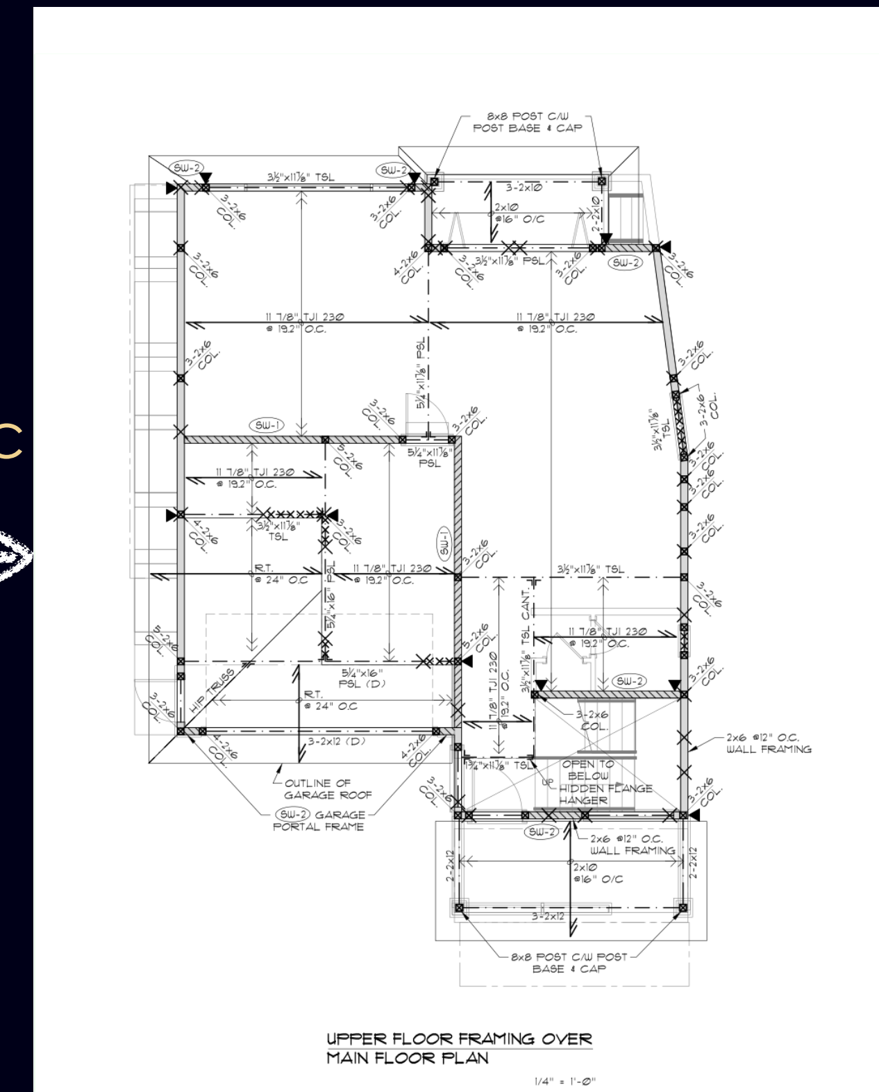
Structural Drawings
